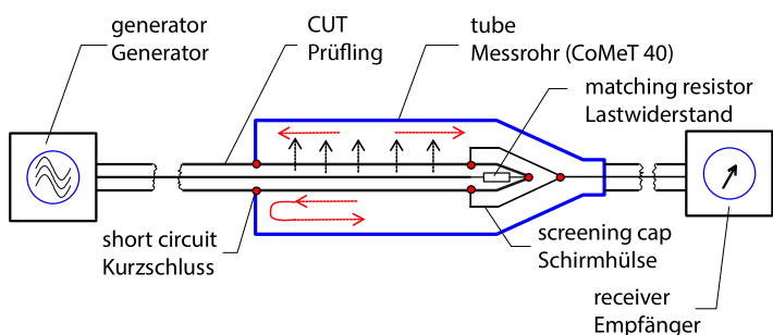
IEC 62153-4-3/-4 Ed.2: Transfer Impedance Z_T & Screening Attenuation a_S Kopplungswiderstand Z_T & Schirmdämpfung a_S
